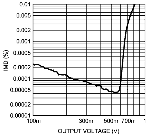
IMD vs Output Voltage V_{CC} = 2.5V, V_{EE} = -2.5V R_L = 600\Omega
